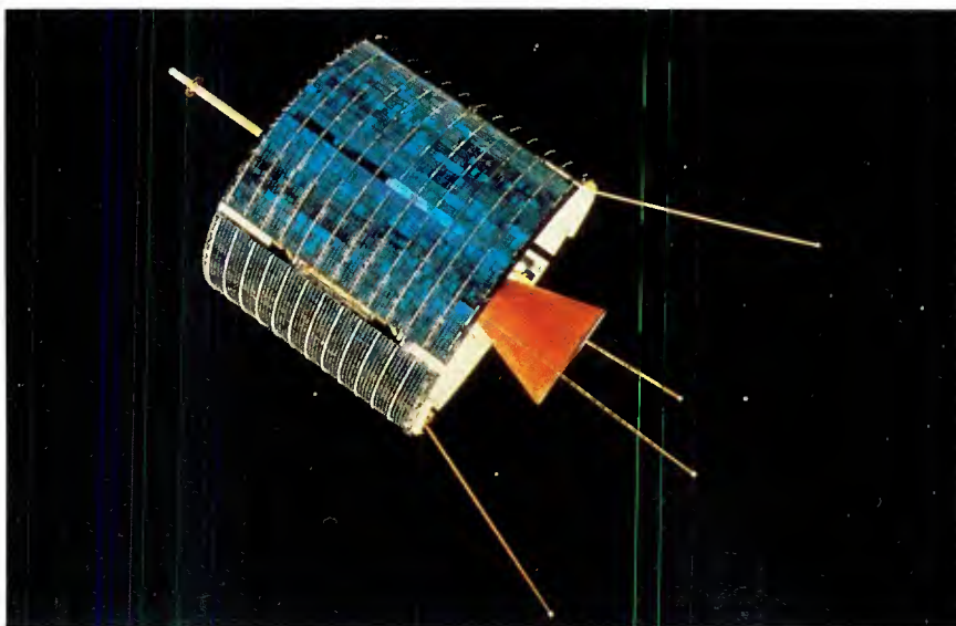
Intelsat I (Early Bird), the world's first commercial communications satellite, was placed in service in April 1965. It established the first satellite pathway between the United States and Europe and made live trans-Atlantic TV possible. (Courtesy of Comsat.)
